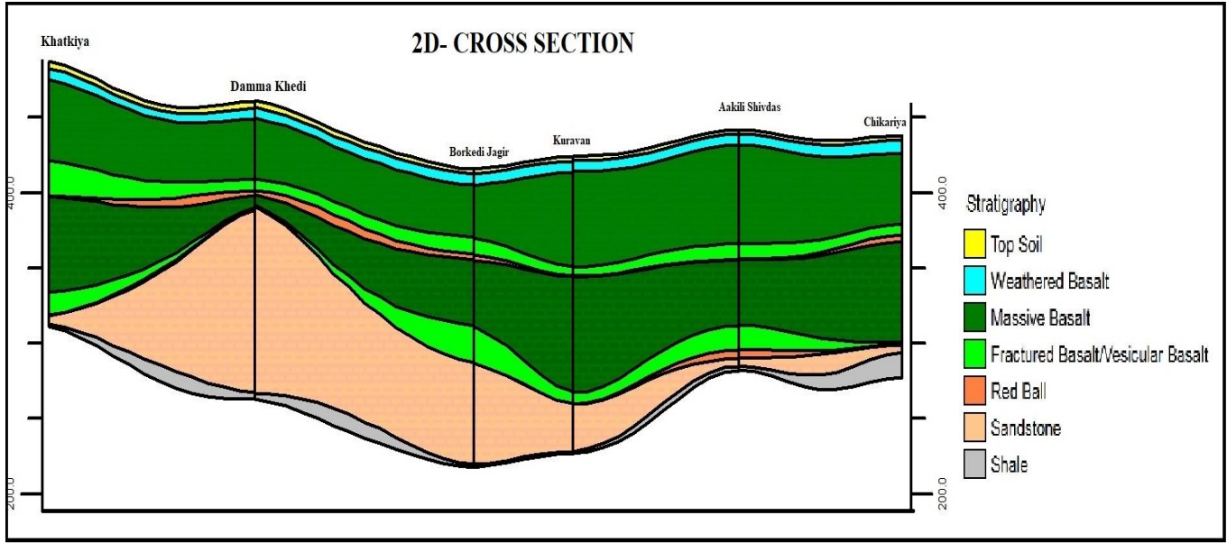
Fig.16 2D- Cross section-I of Mandsaur District
