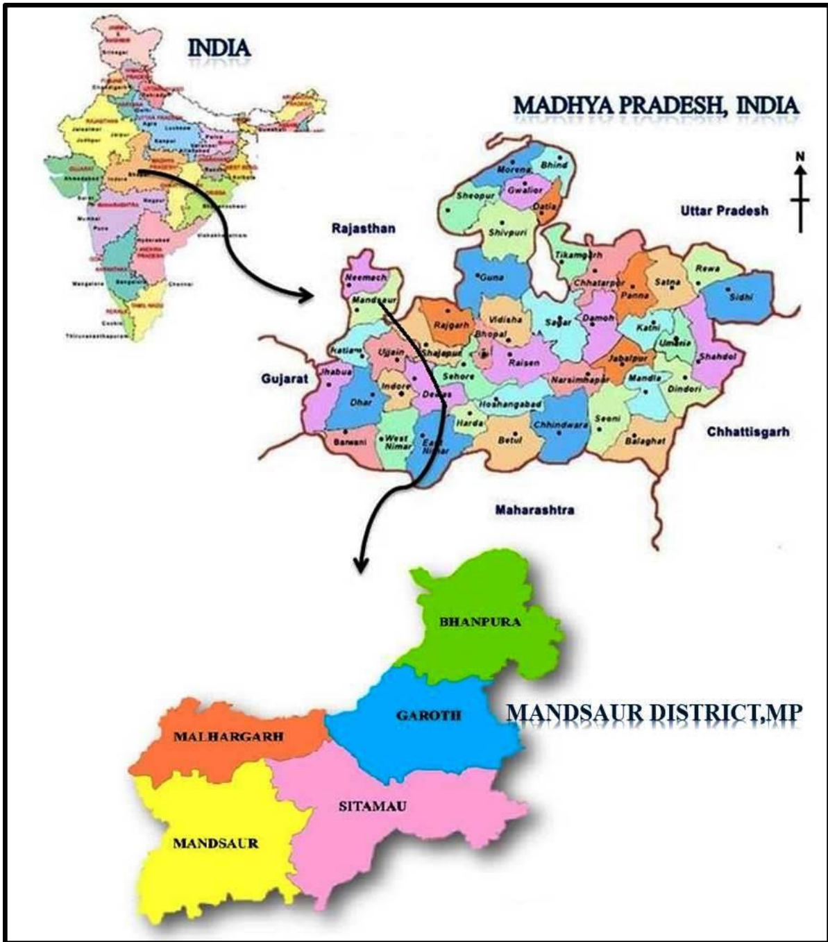
Fig.1 Index Map of Mandsaor District
