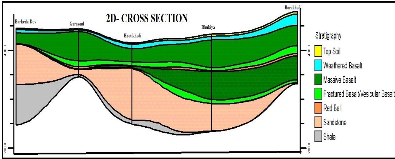
Fig.17 2D- Cross Section-II of Mandsaur District
